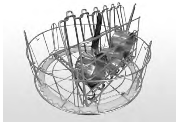
Fig. 14 Multiflex holder
