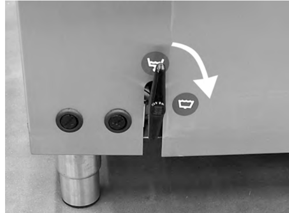
Fig. 3 Drain valve
