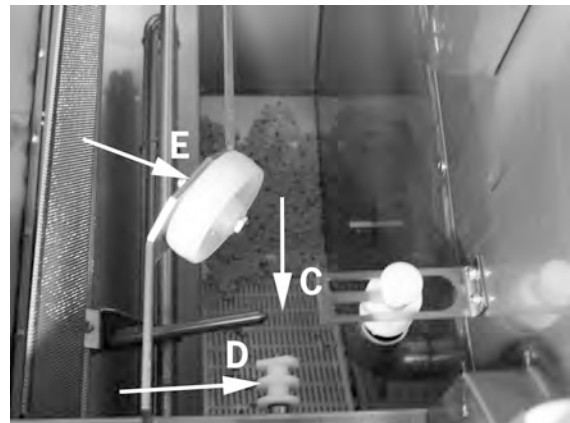
Fig. 40 Bottom sieve, level sensor and rollers
