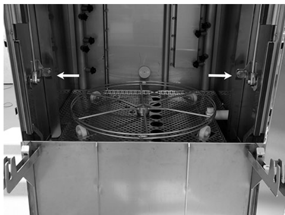
Fig. 32 Lowered door
